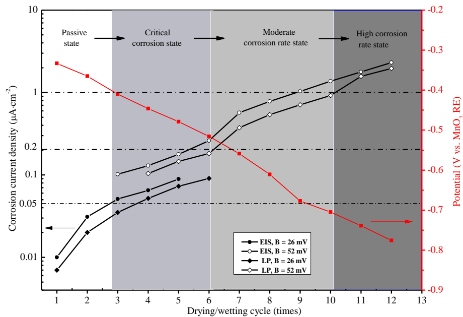
Figure 10. The evolution of half-cell potential (HCP) as well as steel state with the drying/wetting cycle.
