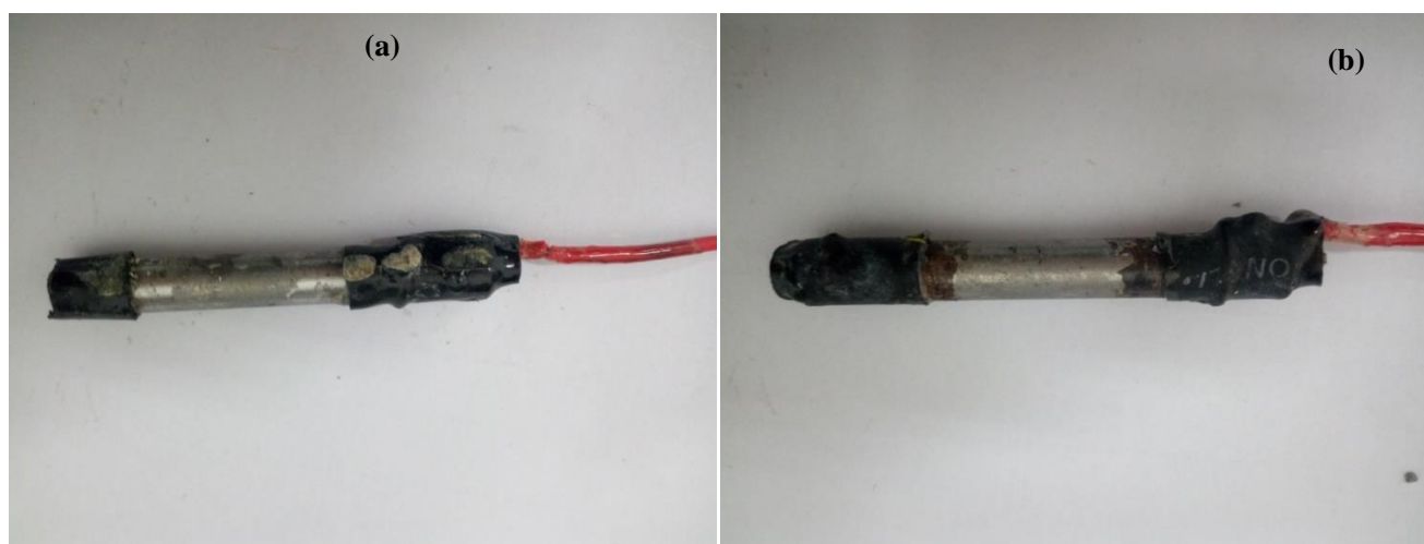
Figure 12. The surface morphologies of steel in concrete after different drying/wetting cycles. (a) cycle 6, and (b) cycle 12.
