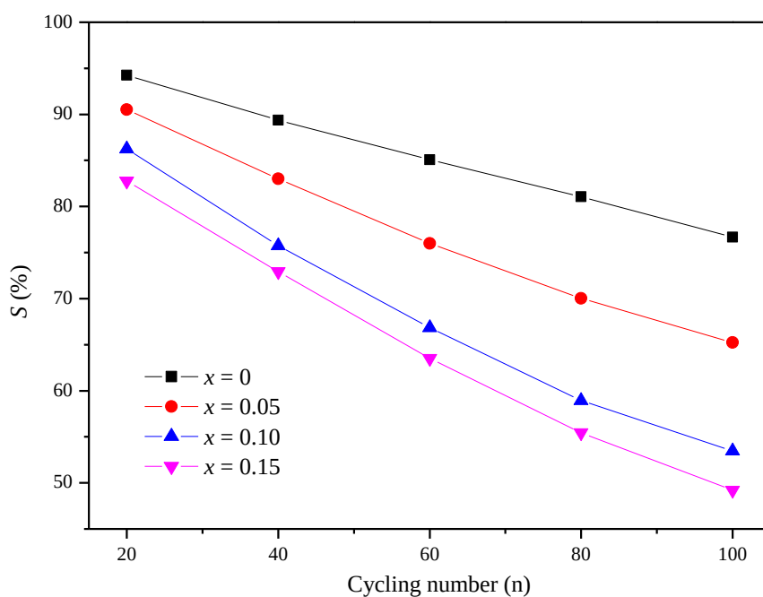
Figure 6. Cycling stability of La_{0.7}Ce_{0.3}Ni_{3.85}Mn_{0.8}Cu_{0.4}Fe_{0.15-x}(Fe_{0.43}B_{0.57})_x alloy electrodes
