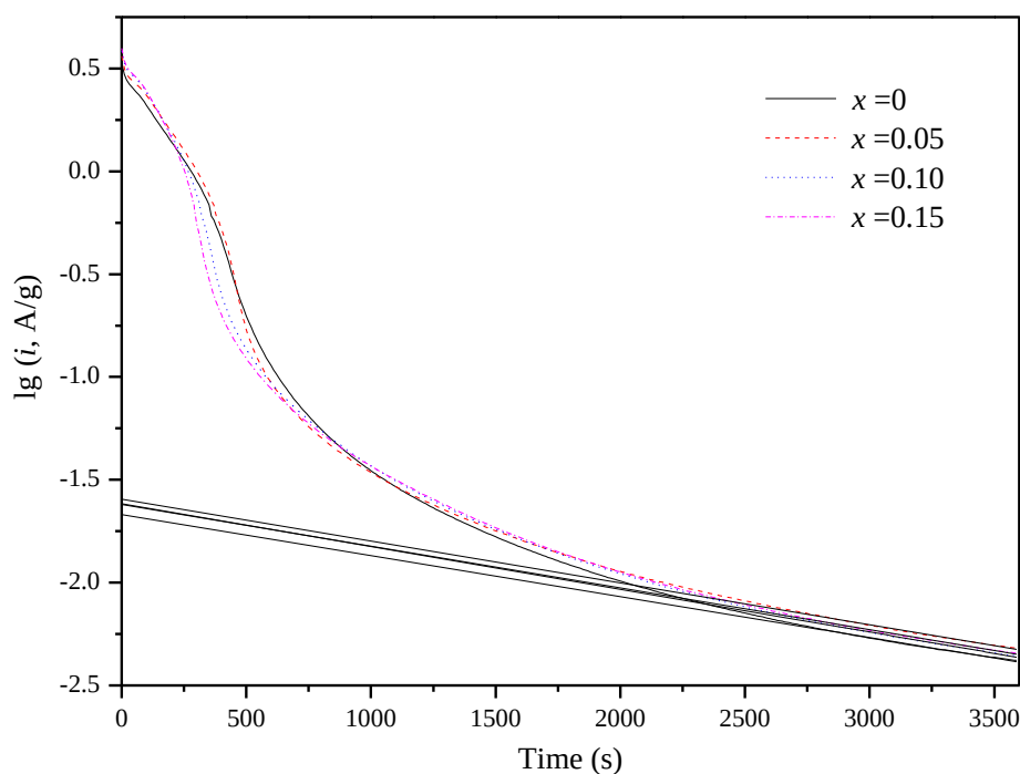
Figure 4. Semilogarithmic curves of anodic current vs. time response of \text{La}_{0.7}\text{Ce}_{0.3}\text{Ni}_{3.85}\text{Mn}_{0.8}\text{Cu}_{0.4}\text{Fe}_{0.15-x}(\text{Fe}_{0.43}\text{B}_{0.57})_x alloy electrodes
