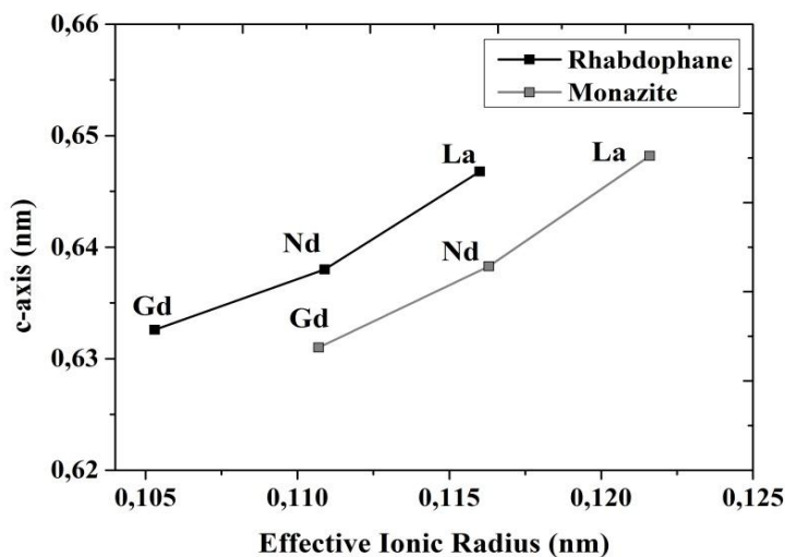
Figure 2. a-axes (a) and c-axes (b) of the rhabdophane MPO_4 \cdot nH_2O and monazite MPO_4 unit cells plotted against effective ionic radius of the corresponding lanthanide.
