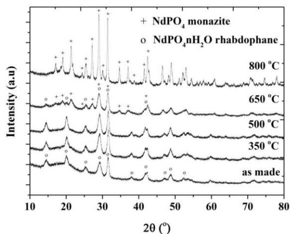
Figure 3. X-ray diffraction patterns of NdPO_4 \cdot nH_2O powders as prepared and heat treated at different temperatures each for a period of 6 hours. Indexing for rhabdophane [21] and monazite [25] structures is indicated in the figure.
